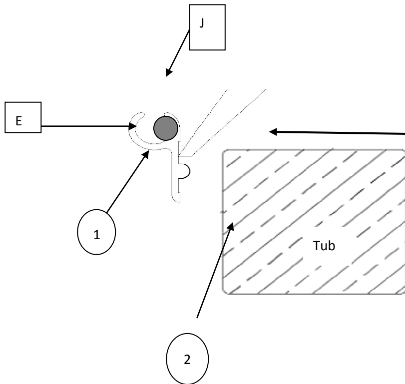
Figure 1 Placement of aluminium rope track. Ensure channel is above the tub's top edge.
