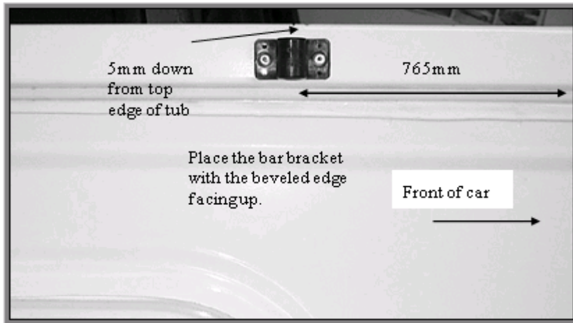
Figure 2: Placement of bar bracket
